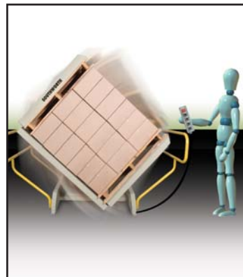
3. Use remote control to clamp and rotate load in about 15 seconds.
